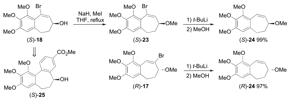
Scheme 6.
