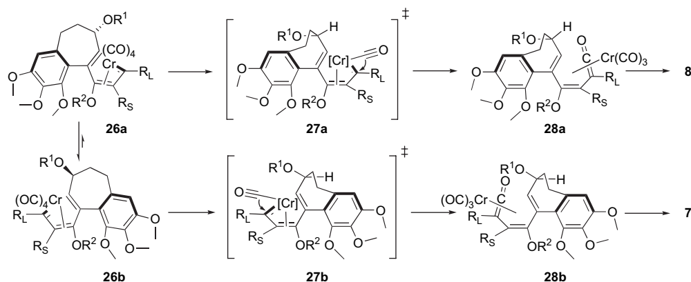
Scheme 8.
