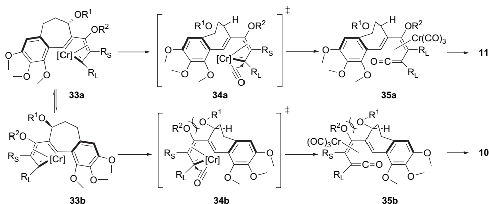
Scheme 10.
